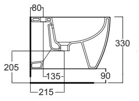
Art. 0750 Bidet sospeso Soho Soho wall hung bidet bowl
