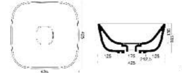
Art. 3141 Vanity Small 42,5x42,5 cm.appoggio Vanity Small counter top basin 42,5x42,5 cm.
