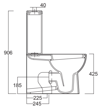
Art. 0250 Vaso monoblocco Soho Soho wc monobloc
