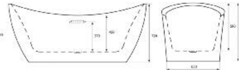
Art. V0518 Vasca in Lucite centrostanza da 180 cm. Center-room Lucite bathtub 180 cm.
