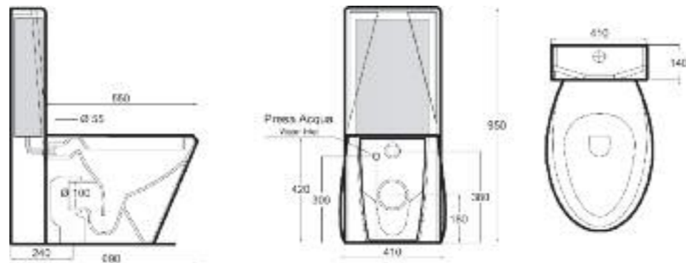
Art. 0352 Cassetta monoblocco a colonna per vaso a terra. Column cistern monoblock for wc back to wall.
