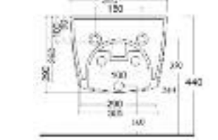
Art. 0752 Bidet sospeso Broadway Broadway wall hung bidet bowl
