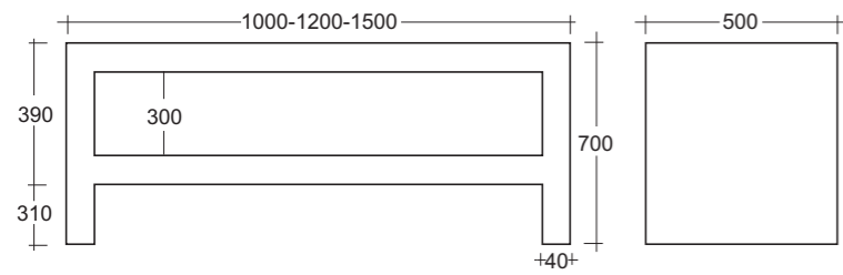
Mobile a terra cm.100x50h70 rovere sbiancato/rovere vengè /bianco lucido/ bianco opaco /beige Floor standing furniture unit cm.100x50h70 bleached oak/vengè oak/white/ matt white/beige
