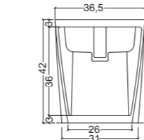
Art. 0552 Bidet Broadway Broadway bidet
